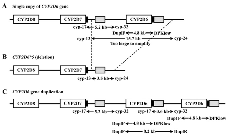
Figure 1. Schematic overview of the CYP2D genes and methods for the detection of CYP2D6 *5 and CYP2D6 gene duplication. Large boxes represent the CYP2D genes. Small black and gray boxes represent 0.6 kb repeats and 2.8 kb CYP-REP units, respectively. The 2.8 kb CYP-REP units are almost completely identical the downstream of the CYP2D7 and CYP2D6 gene and duplicated CYP2D6 gene. The 0.6 kb repeats and 2.8 kb CYP-REP units the downstream of the CYP2D7 gene are separated by a 1.6 kb DNA fragment. The horizontal arrowheads show specific primer sets. (A) For individuals carrying single copy of CYP2D6 gene, 5.2 kb fragment and 4.8 kb fragment are amplified by primer sets, cyp-17 and cyp-32, and DuplF and DPKlow, respectively. The 15.7 kb fragment is too large to amplify with primers cyp-13 and cyp-24. (B) When the CYP2D6 gene is deleted ( CYP2D6 *5), a 3.5 kb fragment is amplified with primers cyp-13 and cyp-24. (C) When duplicated or multiduplicated CYP2D6 genes are present, a 3.6 kb and a 5.2 kb fragment are co-amplified with primers cyp-17 and cyp-32. The 4.8 kb fragment for the presence of the CYP2D6 gene may be potential mixture of PCR products of duplicated and single copy of the CYP2D6 gene. An 8.2 kb fragment yielded by primers DuplF and DuplR only contains the upstream and central CYP2D6 genes.
